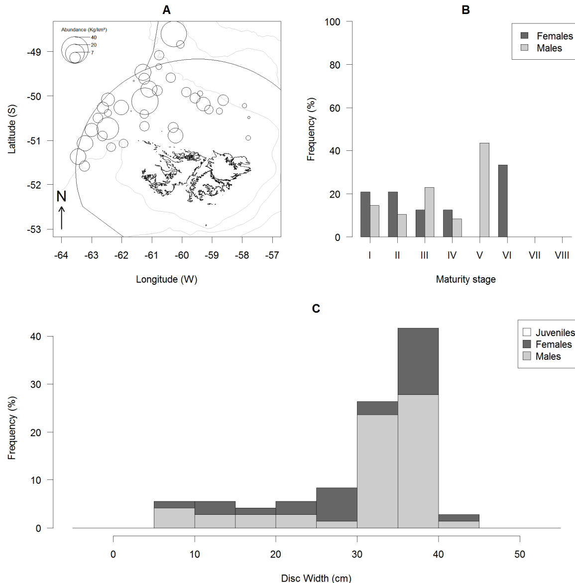
Figure 30: Biological data of Bathyrāja macloviana (Falkland skate, RMC), map of the densities in kg.km -2 (A), percentage of specimens of each sex per maturity stage (B; I, juvenile; II, adolescent, maturing; III, adult, developing; IV, adult, mature; V, adult, laying; VI, adult, resting) and length frequency (in percentage of the total sample assessed) of each sex with 5 cm size class (C).
