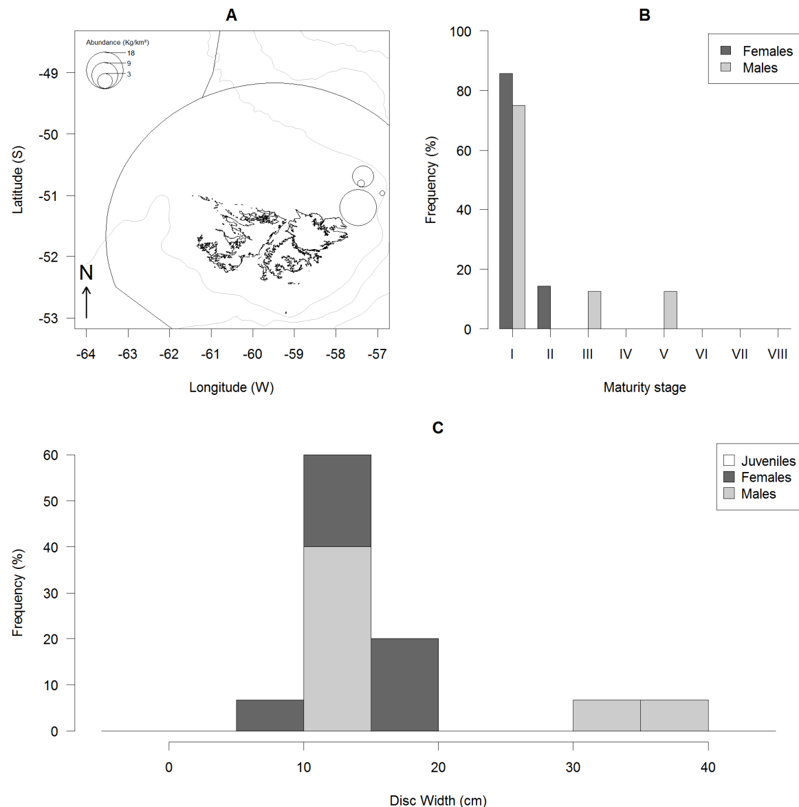
Figure 36: Biological data of Bathyrāja magellanica (Magellanic skate, RMG), map of the densities in kg.km -2 (A), percentage of specimens of each sex per maturity stage (B; I, juvenile; II, adolescent, maturing; III, adult, developing; IV, adult, mature; V, adult, laying; VI, adult, resting) and length frequency (in percentage of the total sample assessed) of each sex with 5 cm size class (C).
