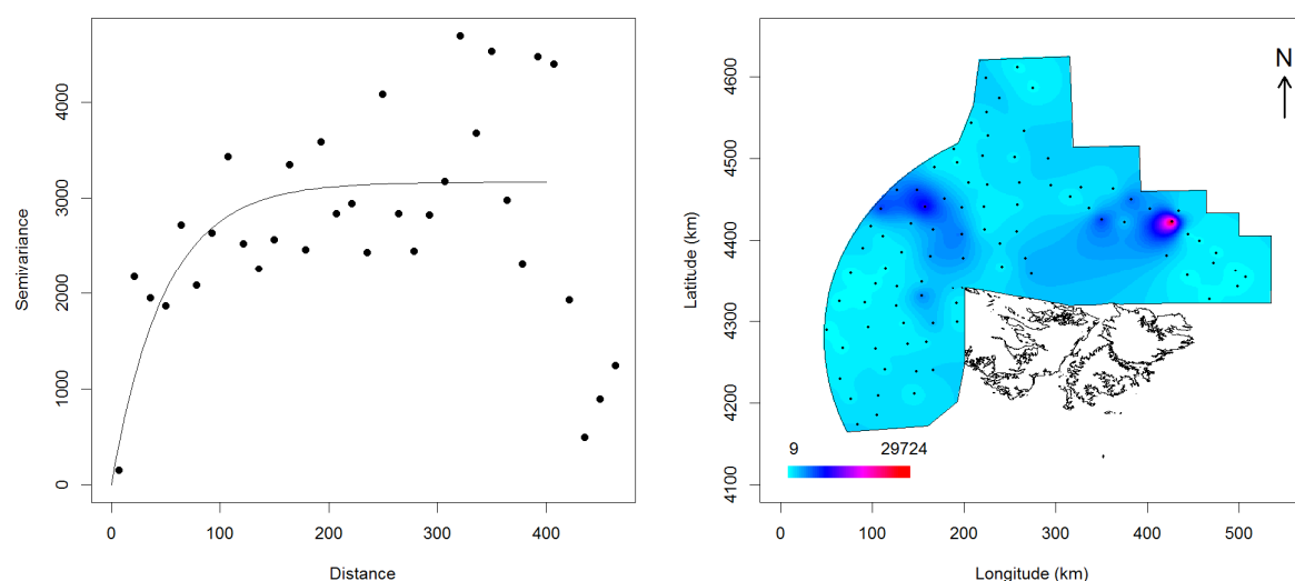
Figure 41: Experimental variogram (dots) and exponential variogram model (line) of the ZDLT1-02-2016 survey (left) and krige map of density with legend in \text{kg.km}^{-2} (right).
