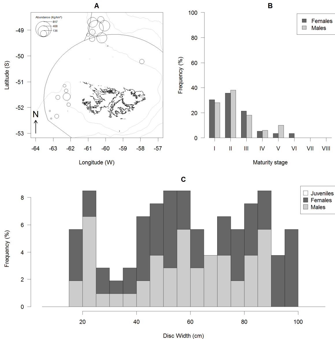
Figure 26: Biological data of Bathyrāja griseocauda (grey tailed skate, RGR), map of the densities in kg.km -2 (A), percentage of specimens of each sex per maturity stage (B; I, juvenile; II, adolescent, maturing; III, adult, developing; IV, adult, mature; V, adult, laying; VI, adult, resting) and length frequency (in percentage of the total sample assessed) of each sex with 5 cm size class (C).
