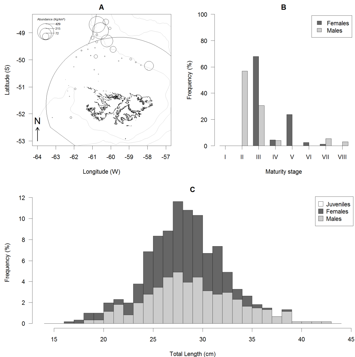
Figure 12: Biological data of Iluocoetes fimbriatus (eelpout, EEL), map of the densities in kg.km -2 (A), percentage of specimens of each sex per maturity stage (B; I, immature; II, resting; III, early developing; IV, late developing; V, ripe; VI, running; VII, spent; VIII, recovering spent) and length frequency (in percentage of the total sample assessed) of each sex with 1 cm size class (C).
