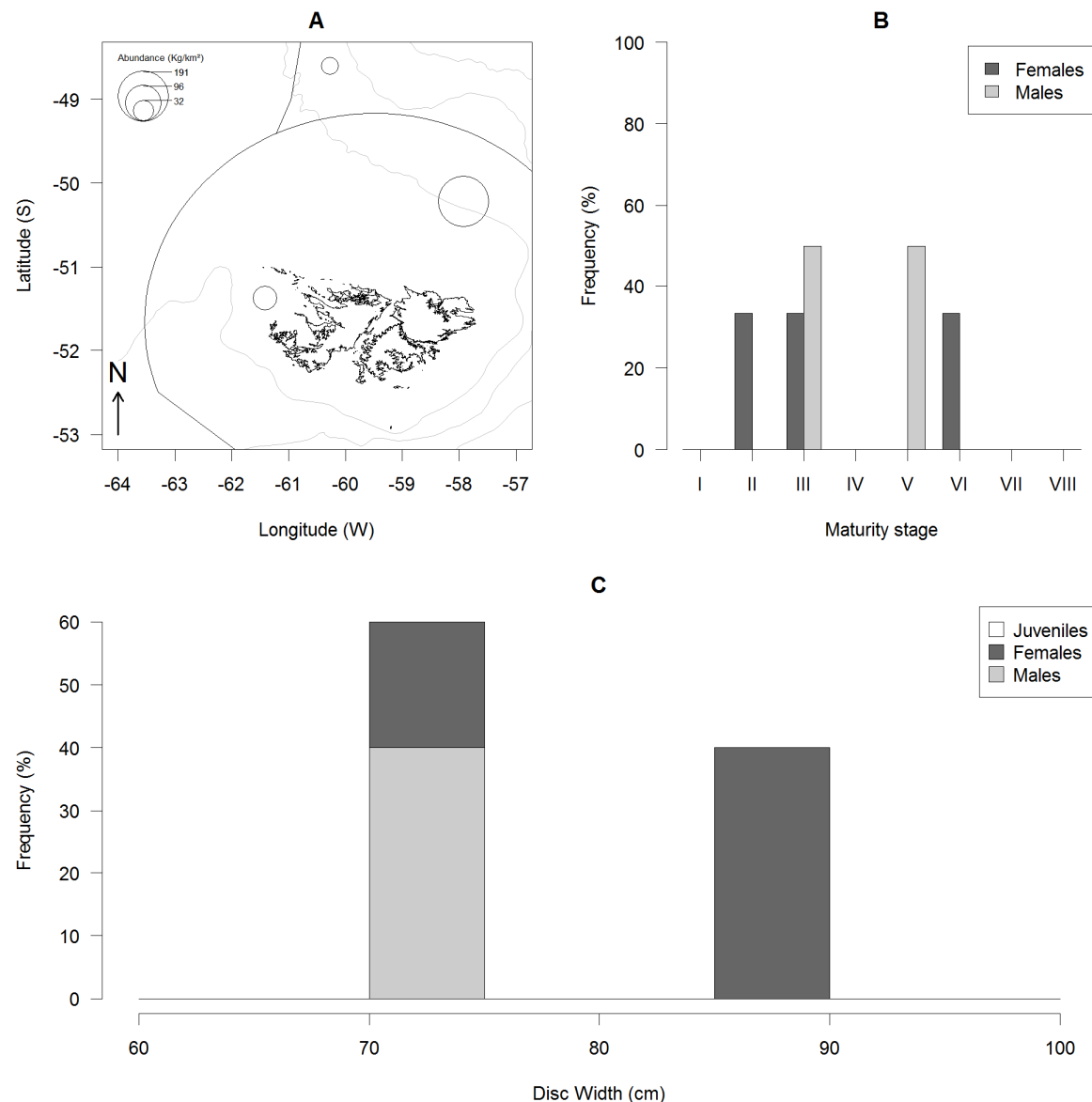
Figure 31: Biological data of Bathyrāja multispinis (multispined skate, RMU), map of the densities in kg.km -2 (A), percentage of specimens of each sex per maturity stage (B; I, juvenile; II, adolescent, maturing; III, adult, developing; IV, adult, mature; V, adult, laying; VI, adult, resting) and length frequency (in percentage of the total sample assessed) of each sex with 5 cm size class (C).
